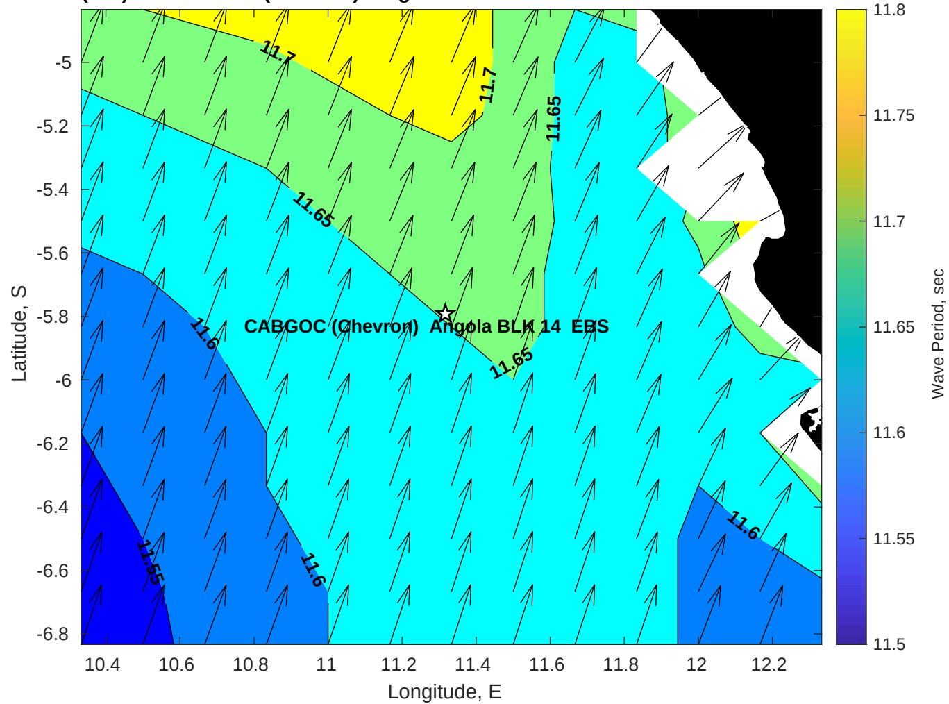
Wave Period (sec) for CABGOC (Chevron) Angola BLK 14 EBS at 01-Jun-2025 09:00:00
