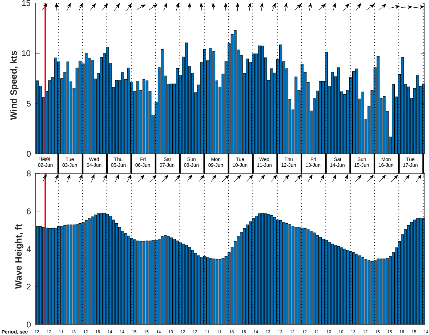
Wind & Wave Forecast for CABGOC (Chevron) Angola BLK 14 EBS from 01-Jun-2025 02:00:00 to 17-Jun-2025 02:00:00
