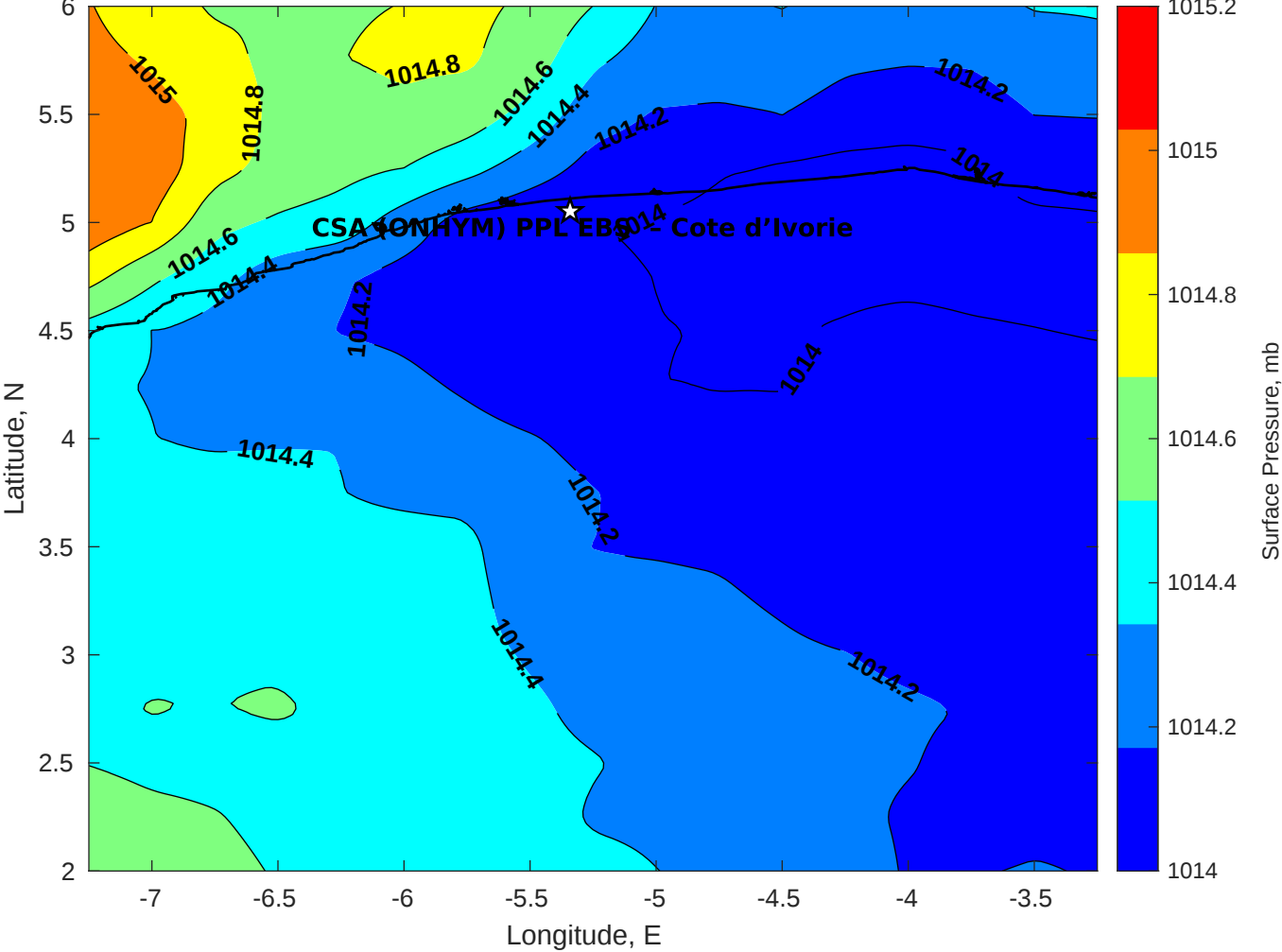
Surface Pressure (mb) for CSA (ONHYM) PPL EBS - Cote d'Ivoire at 01-Jun-2025 00:00:00
