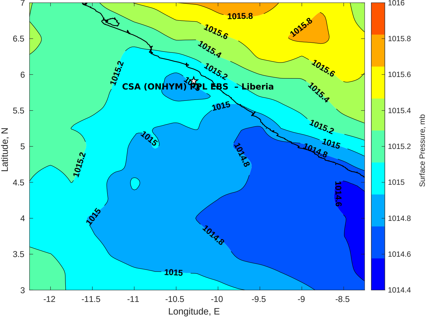
Surface Pressure (mb) for CSA (ONHYM) PPL EBS - Liberia at 01-Jun-2025 00:00:00
