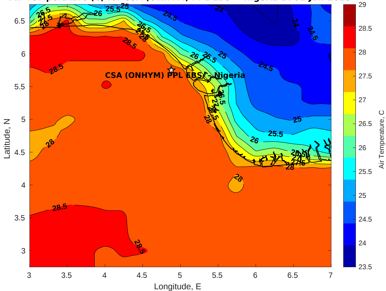
Air Temperature (C) for CSA (ONHYM) PPL EBS - Nigeria at 01-Jun-2025
