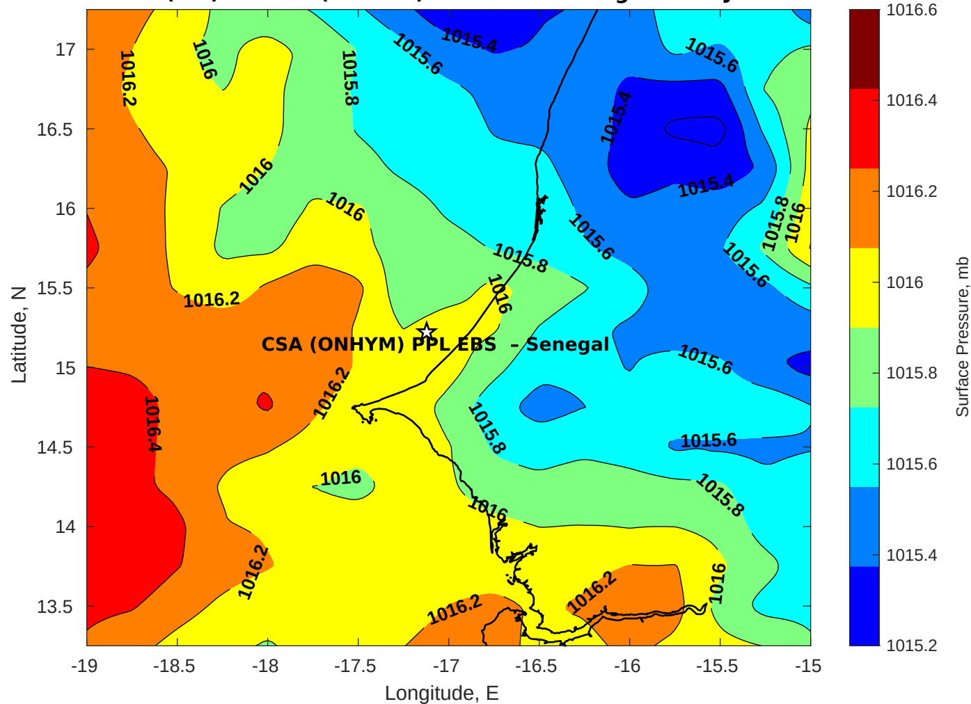
Surface Pressure (mb) for CSA (ONHYM) PPL EBS - Senegal at 01-Jun-2025 00:00:00
