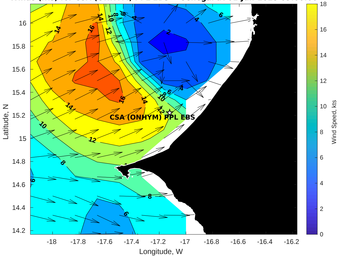
Winds (kts) for CSA (ONHYM) PPL EBS - Senegal at 01-Jun-2025 09:00:00
