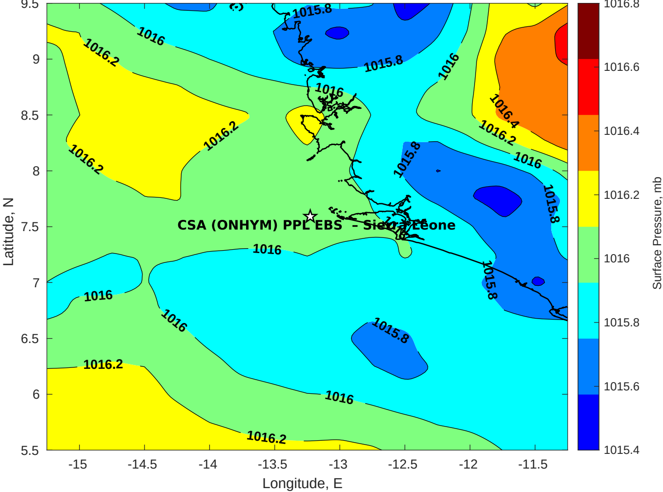
Surface Pressure (mb) for CSA (ONHYM) PPL EBS - Sierra Leone at 03-Jun-2025 00:00:00
