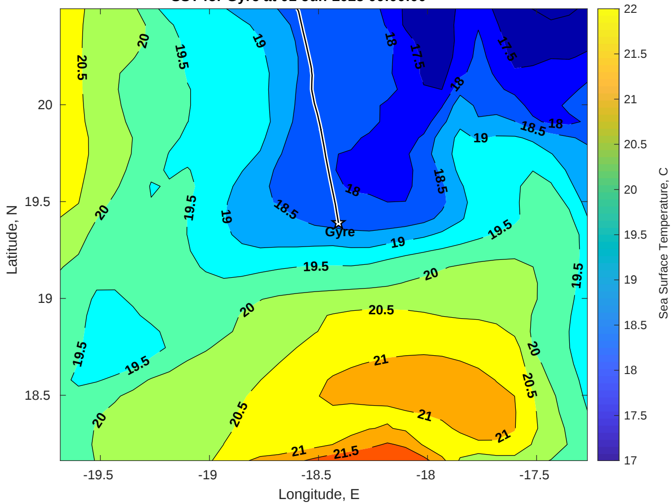
SST for Gyre at 01-Jun-2025 00:00:00
