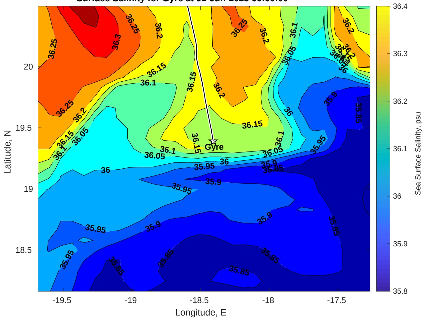
Surface Salinity for Gyre at 01-Jun-2025 00:00:00
