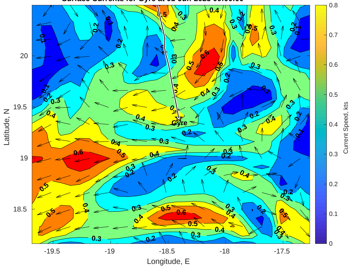
Surface Currents for Gyre at 01-Jun-2025 00:00:00
