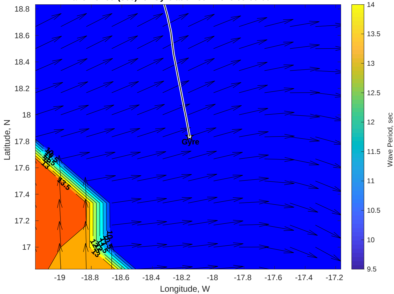
Wave Period (sec) for Gyre at 02-Jun-2025 09:00:00
