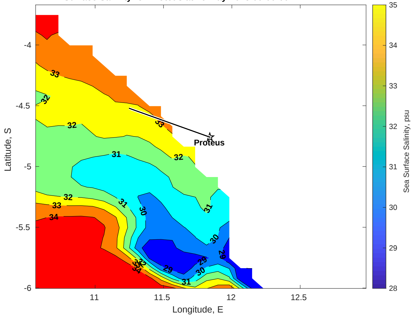
Surface Salinity for Proteus at 26-May-2025 00:00:00
