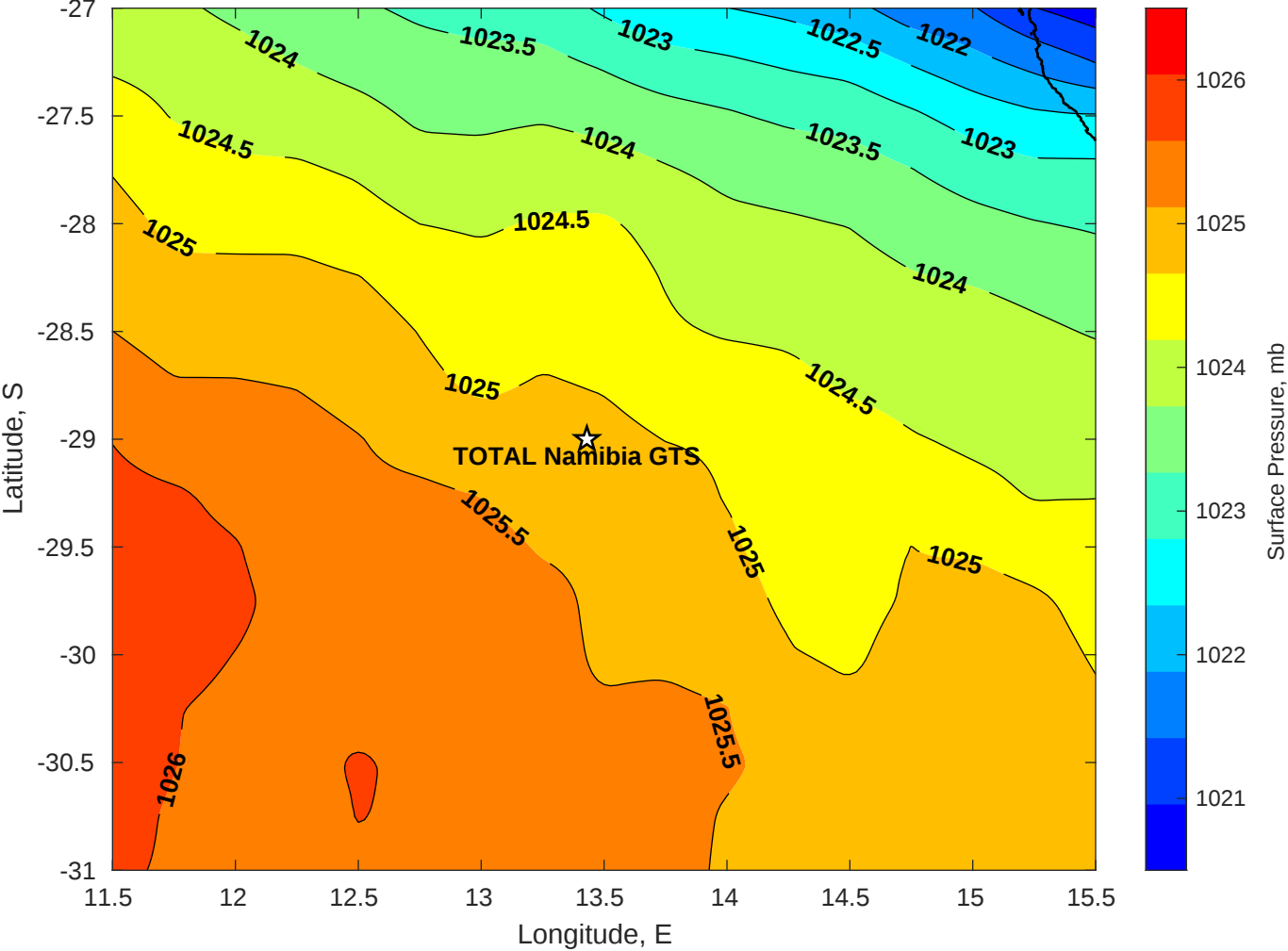
Surface Pressure (mb) for TOTAL Namibia GTS at 01-Jun-2025 00:00:00
