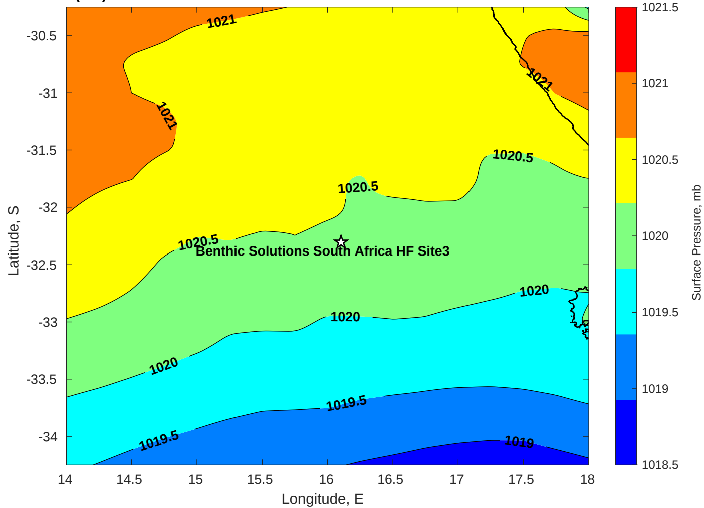
Surface Pressure (mb) for Benthic Solutions South Africa HF Site3 at 03-Jun-2025 00:00:00
