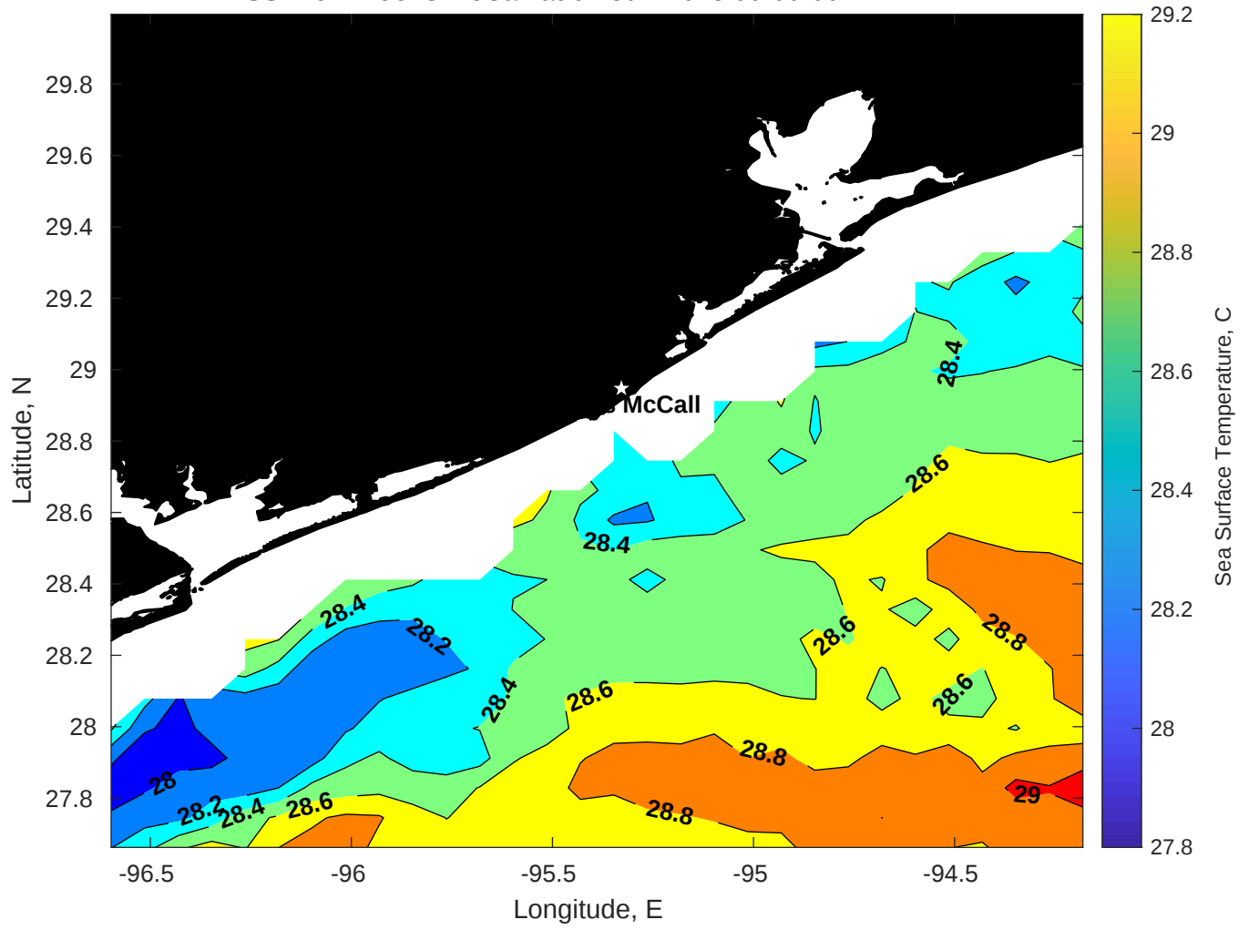
SST for Brooks McCall at 02-Jun-2025 00:00:00
