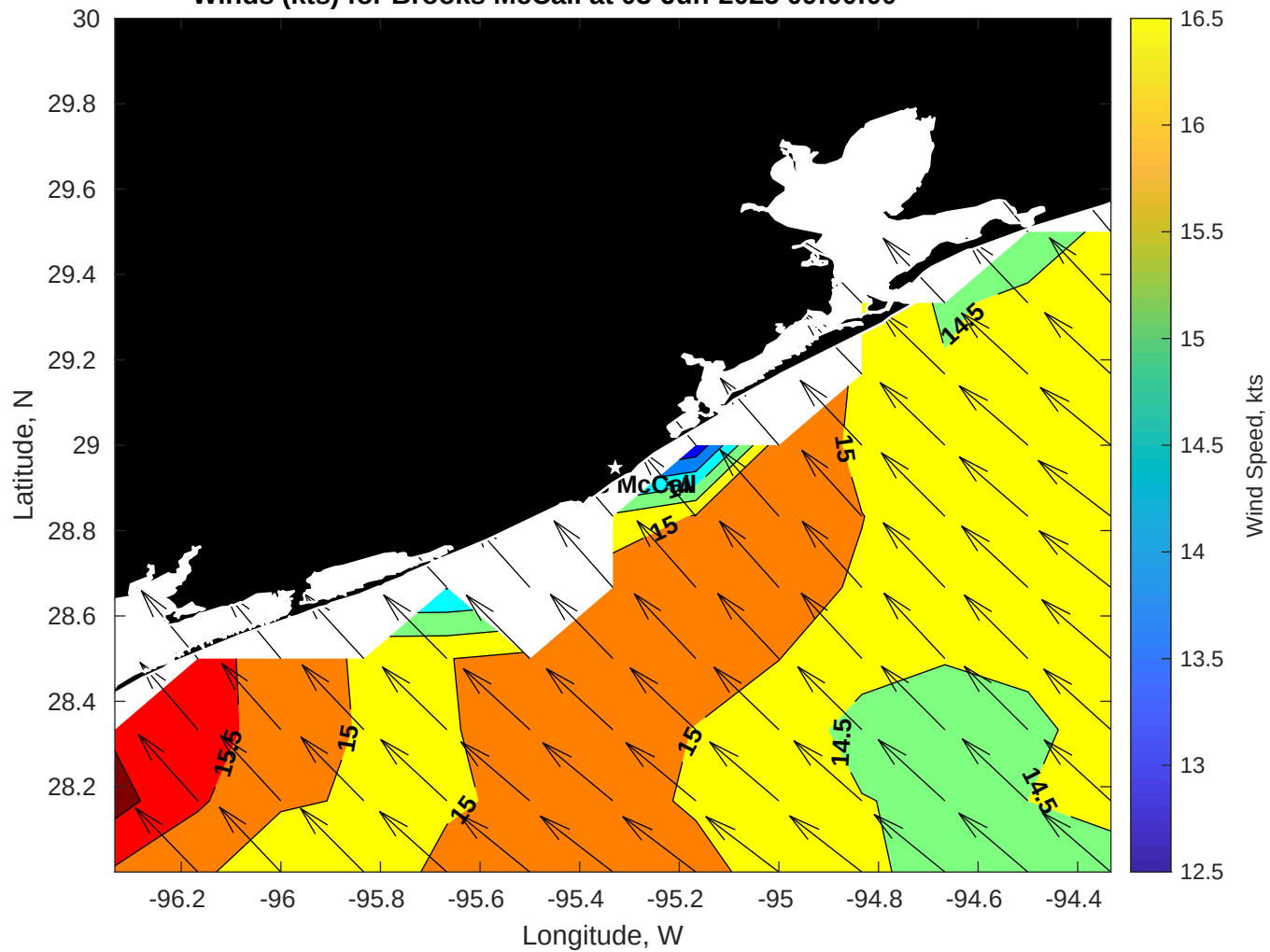
Winds (kts) for Brooks McCall at 03-Jun-2025 09:00:00
