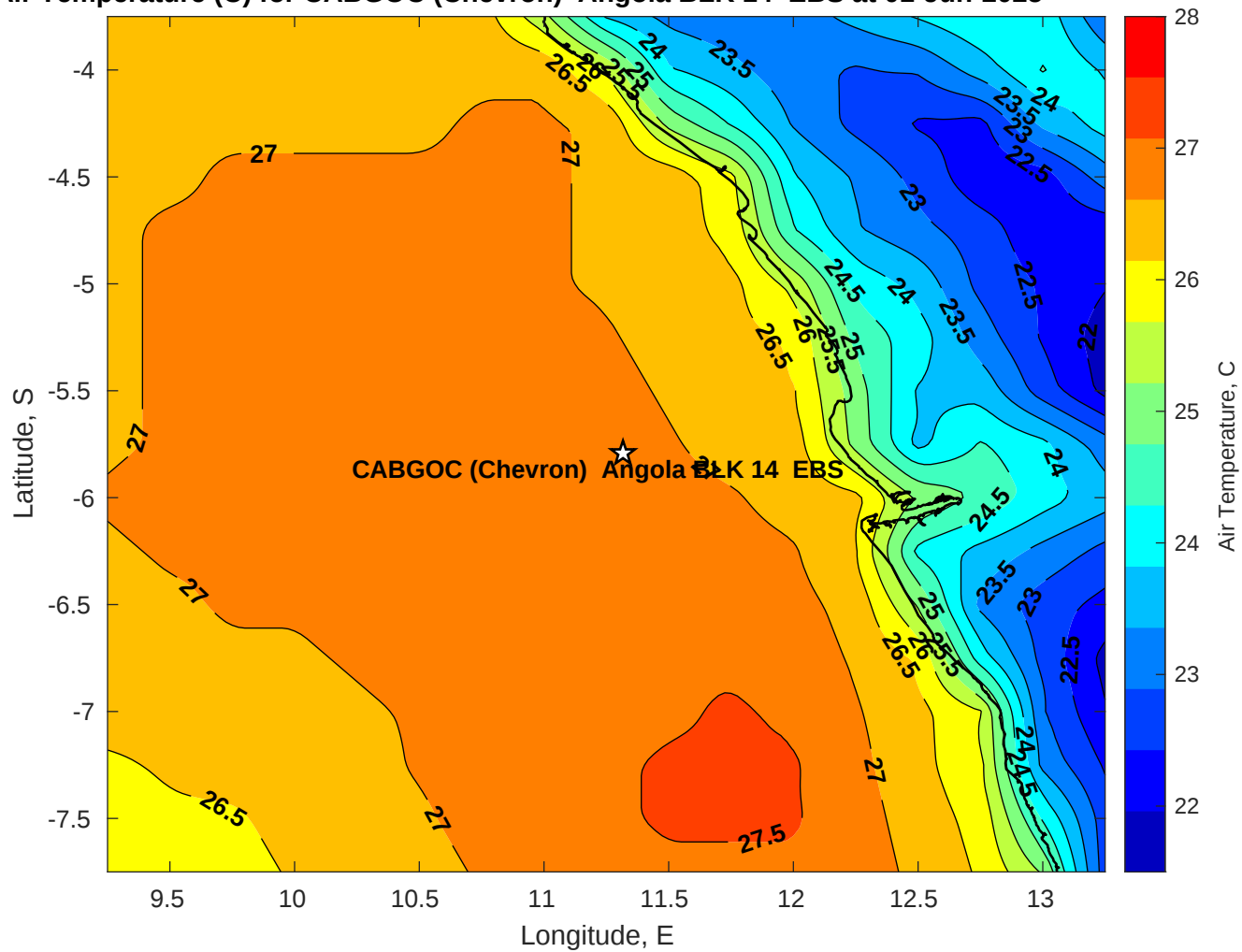
Air Temperature (C) for CABGOC (Chevron) Angola BLK 14 EBS at 01-Jun-2025
