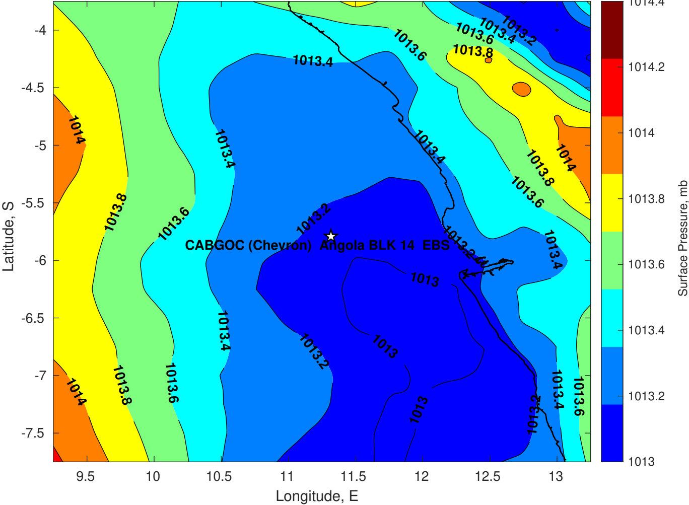
Surface Pressure (mb) for CABGOC (Chevron) Angola BLK 14 EBS at 03-Jun-2025 00:00:00
