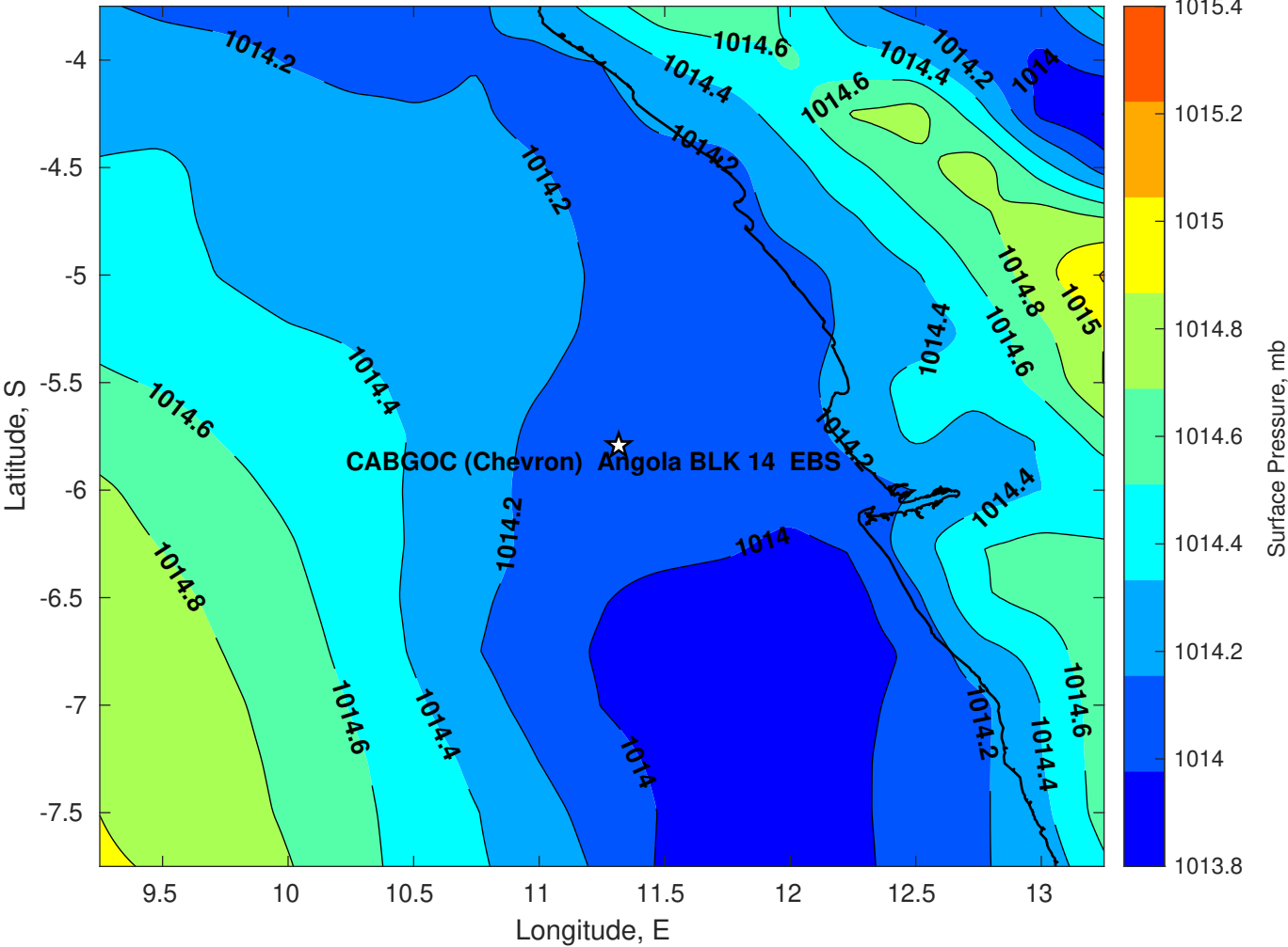
Surface Pressure (mb) for CABGOC (Chevron) Angola BLK 14 EBS at 02-Jun-2025 00:00:00
