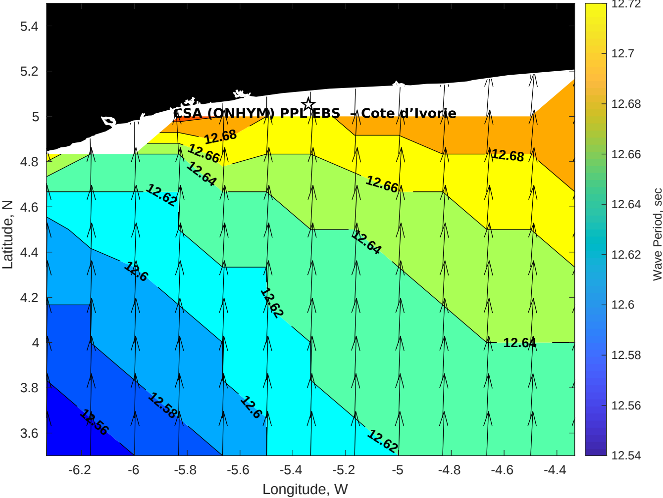
Wave Period (sec) for CSA (ONHYM) PPL EBS - Cote d'Ivoire at 01-Jun-2025 09:00:00
