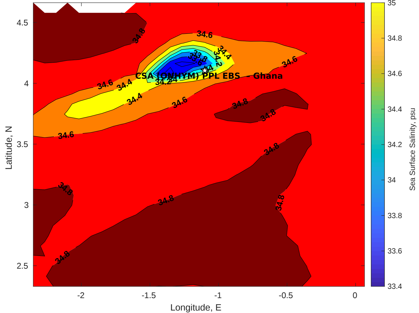
Surface Salinity for CSA (ONHYM) PPL EBS - Ghana at 26-May-2025 00:00:00
