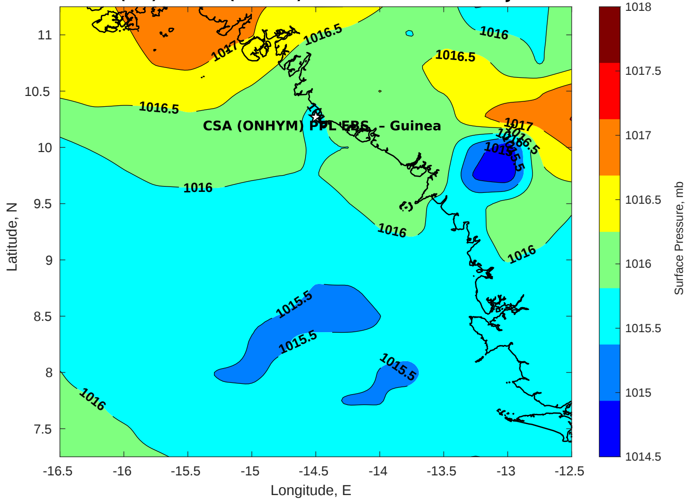
Surface Pressure (mb) for CSA (ONHYM) PPL EBS - Guinea at 02-Jun-2025 00:00:00
