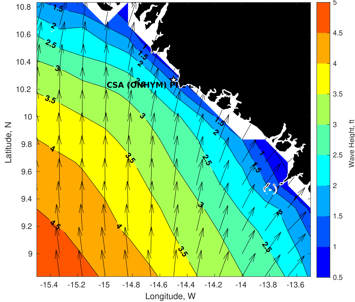
Wave Height (ft) for CSA (ONHYM) PPL EBS - Guinea at 01-Jun-2025 09:00:00
