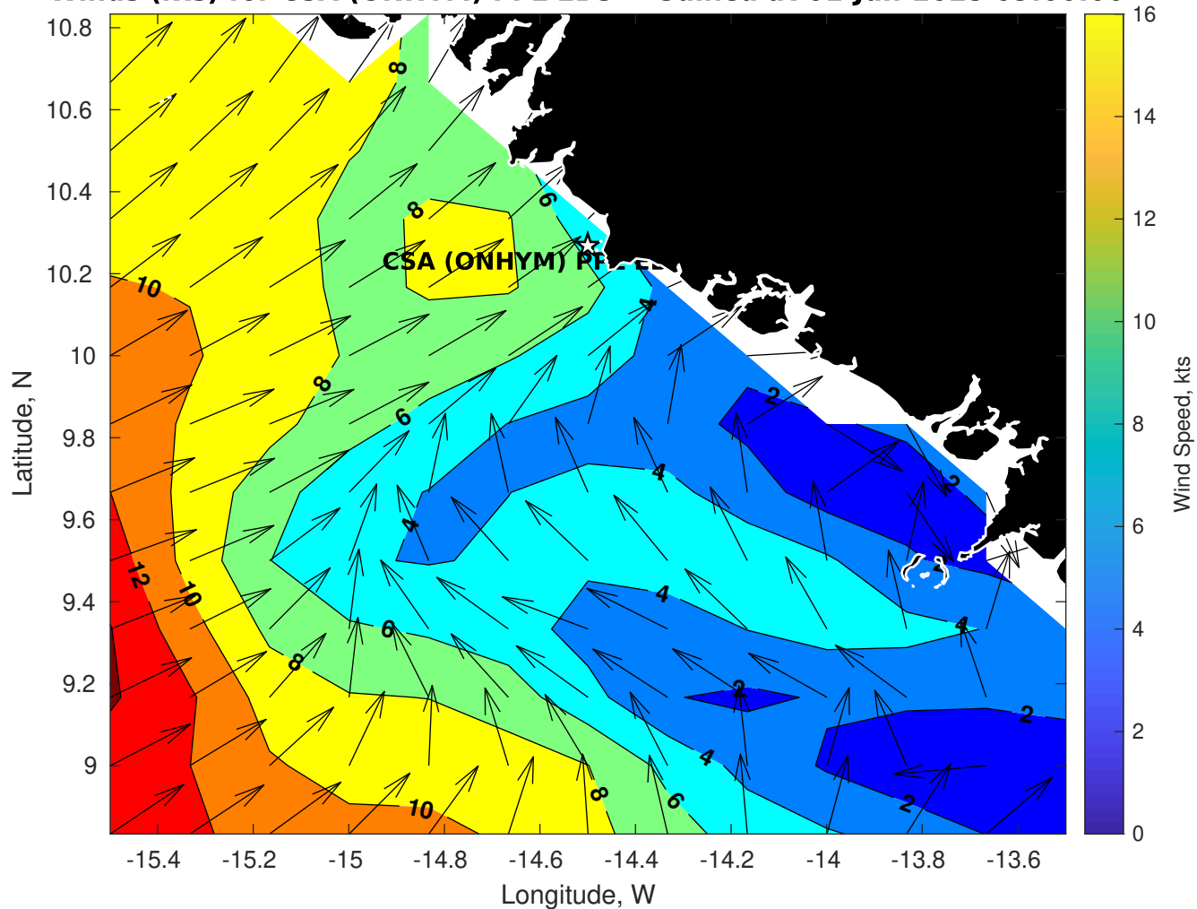
Winds (kts) for CSA (ONHYM) PPL EBS - Guinea at 01-Jun-2025 09:00:00
