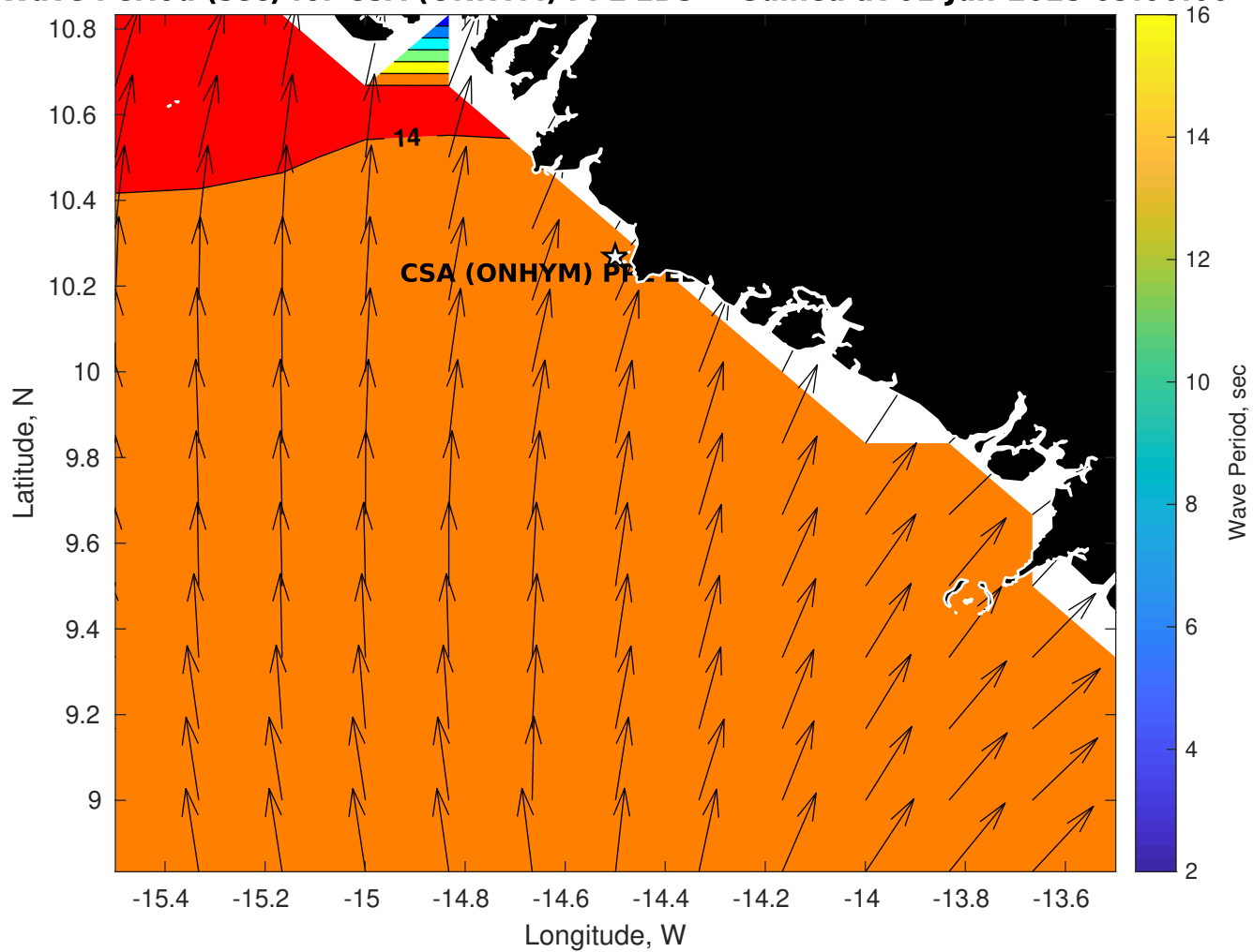
Wave Period (sec) for CSA (ONHYM) PPL EBS - Guinea at 01-Jun-2025 09:00:00
