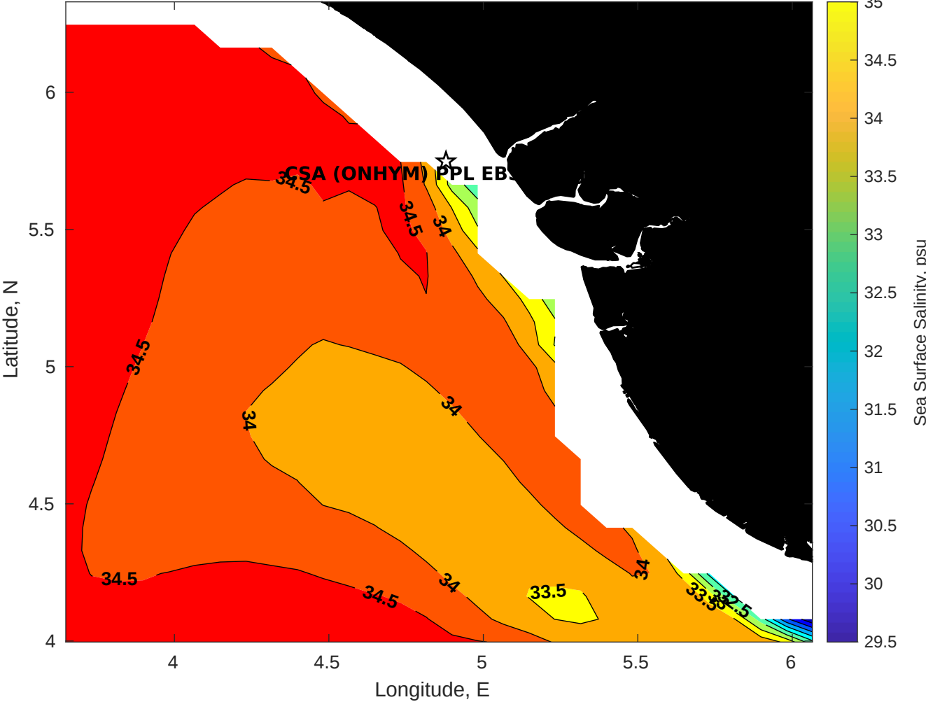
Surface Salinity for CSA (ONHYM) PPL EBS - Nigeria at 26-May-2025 00:00:00
