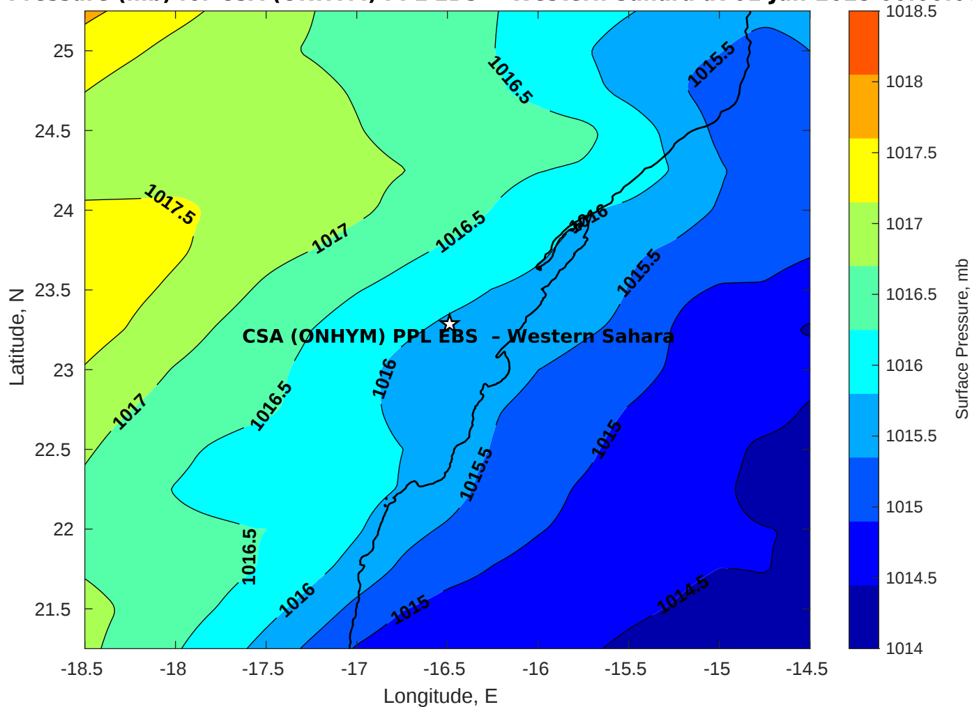
Surface Pressure (mb) for CSA (ONHYM) PPL EBS - Western Sahara at 01-Jun-2025 00:00:00
