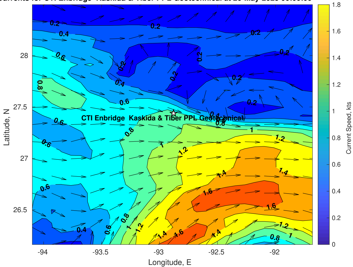
Surface Currents for CTI Enbridge Kaskida & Tiber PPL Geotechnical at 26-May-2025 00:00:00
