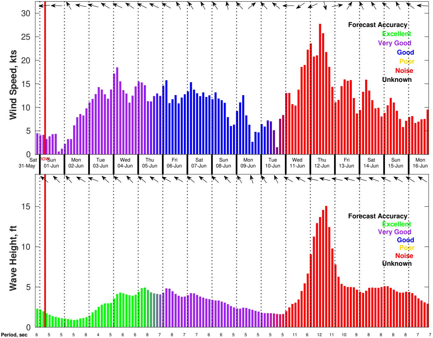
Wind & Wave Forecast for CTI Enbridge Kaskida & Tiber PPL Geotechnical from 31-May-2025 20:00:00 to 16-Jun-2025 20:00:00
