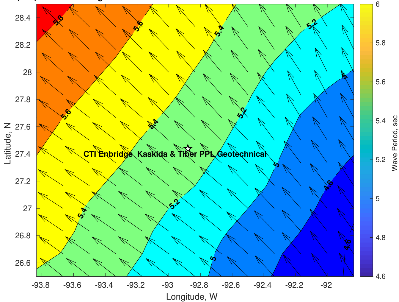
Wave Period (sec) for CTI Enbridge Kaskida & Tiber PPL Geotechnical at 01-Jun-2025 09:00:00
