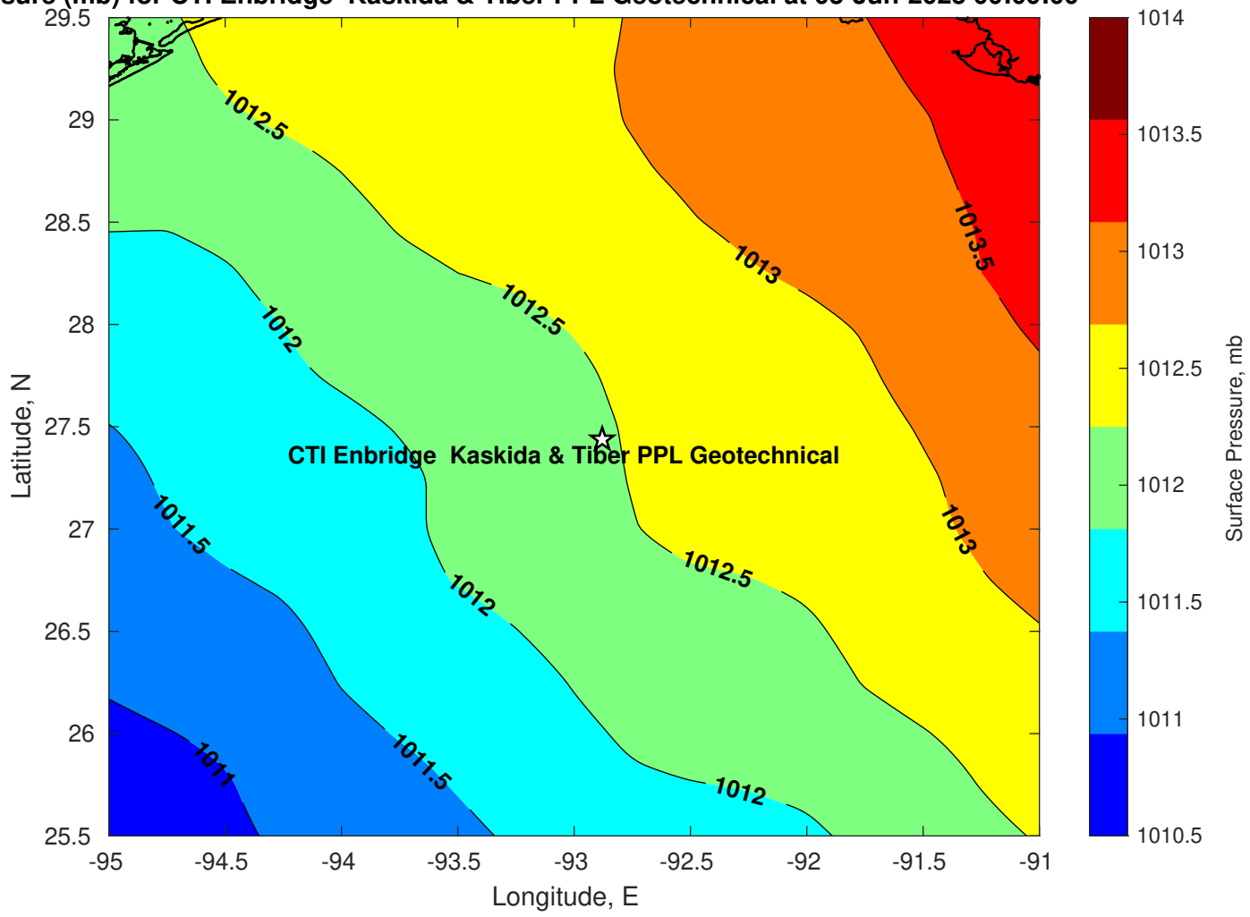
Surface Pressure (mb) for CTI Enbridge Kaskida & Tiber PPL Geotechnical at 03-Jun-2025 00:00:00
