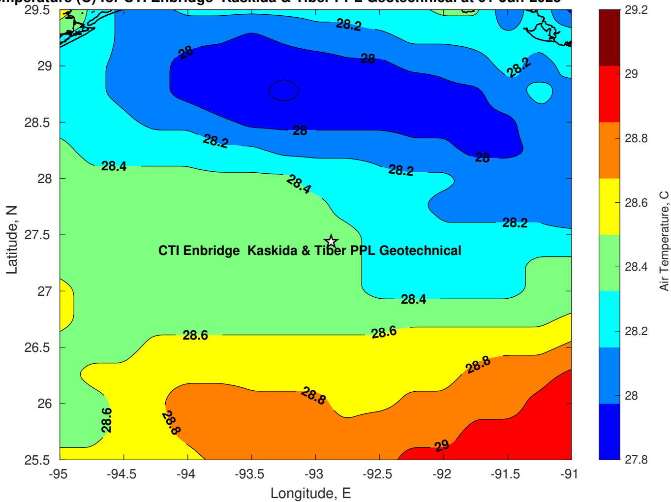
Air Temperature (C) for CTI Enbridge Kaskida & Tiber PPL Geotechnical at 01-Jun-2025
