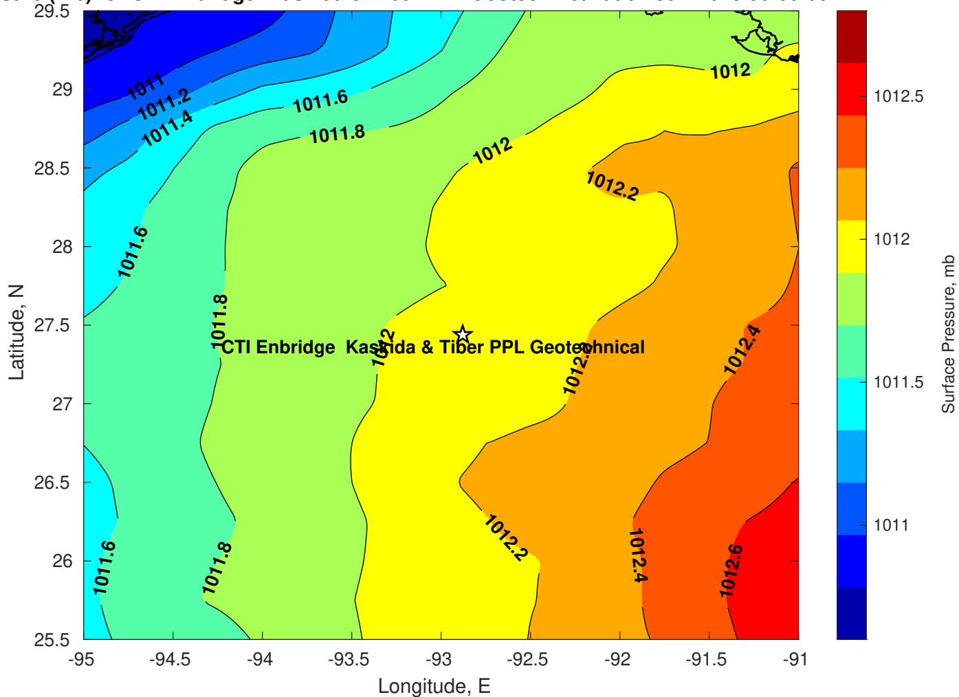
Surface Pressure (mb) for CTI Enbridge Kaskida & Tiber PPL Geotechnical at 02-Jun-2025 00:00:00
