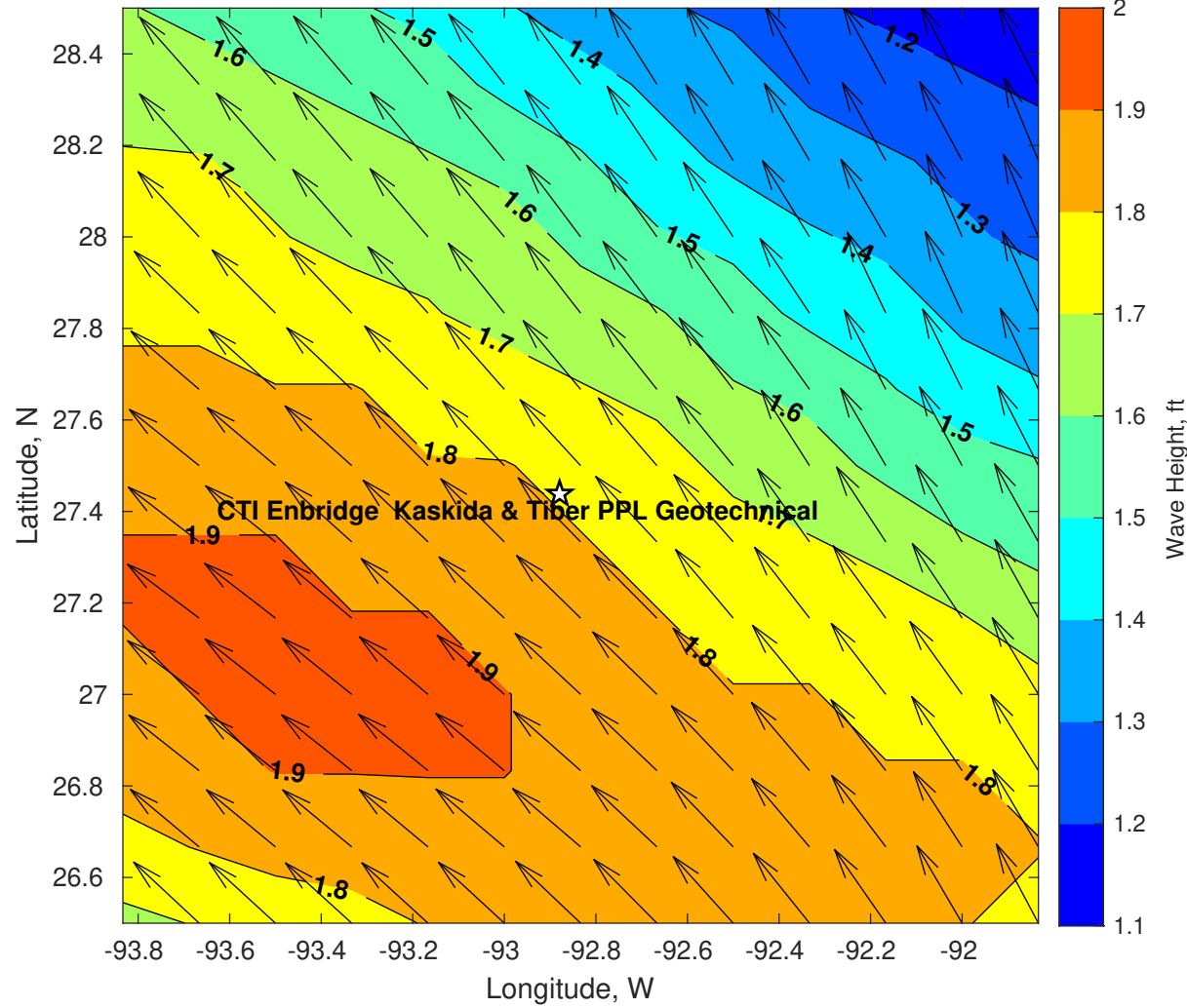
Wave Height (ft) for CTI Enbridge Kaskida & Tiber PPL Geotechnical at 01-Jun-2025 09:00:00
