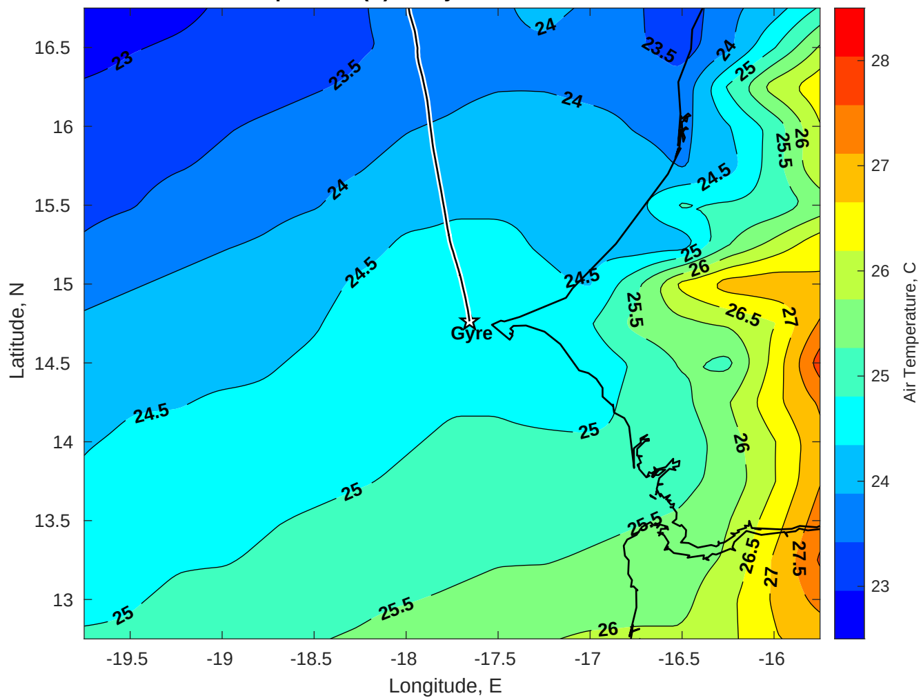
Air Temperature (C) for Gyre at 03-Jun-2025
