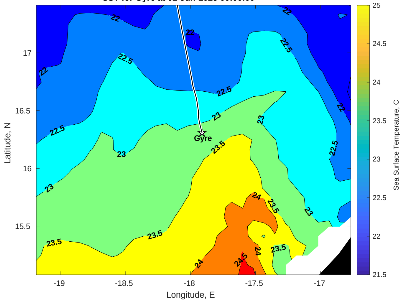
SST for Gyre at 02-Jun-2025 00:00:00
