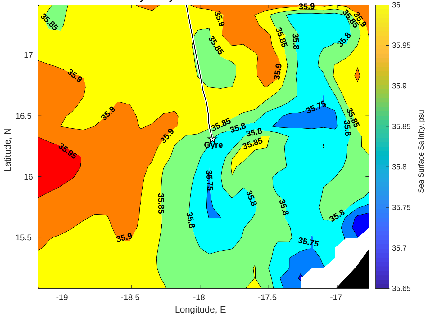
Surface Salinity for Gyre at 02-Jun-2025 00:00:00
