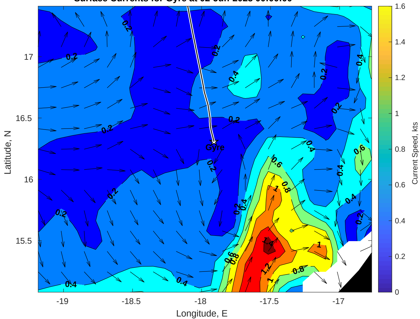
Surface Currents for Gyre at 02-Jun-2025 00:00:00
