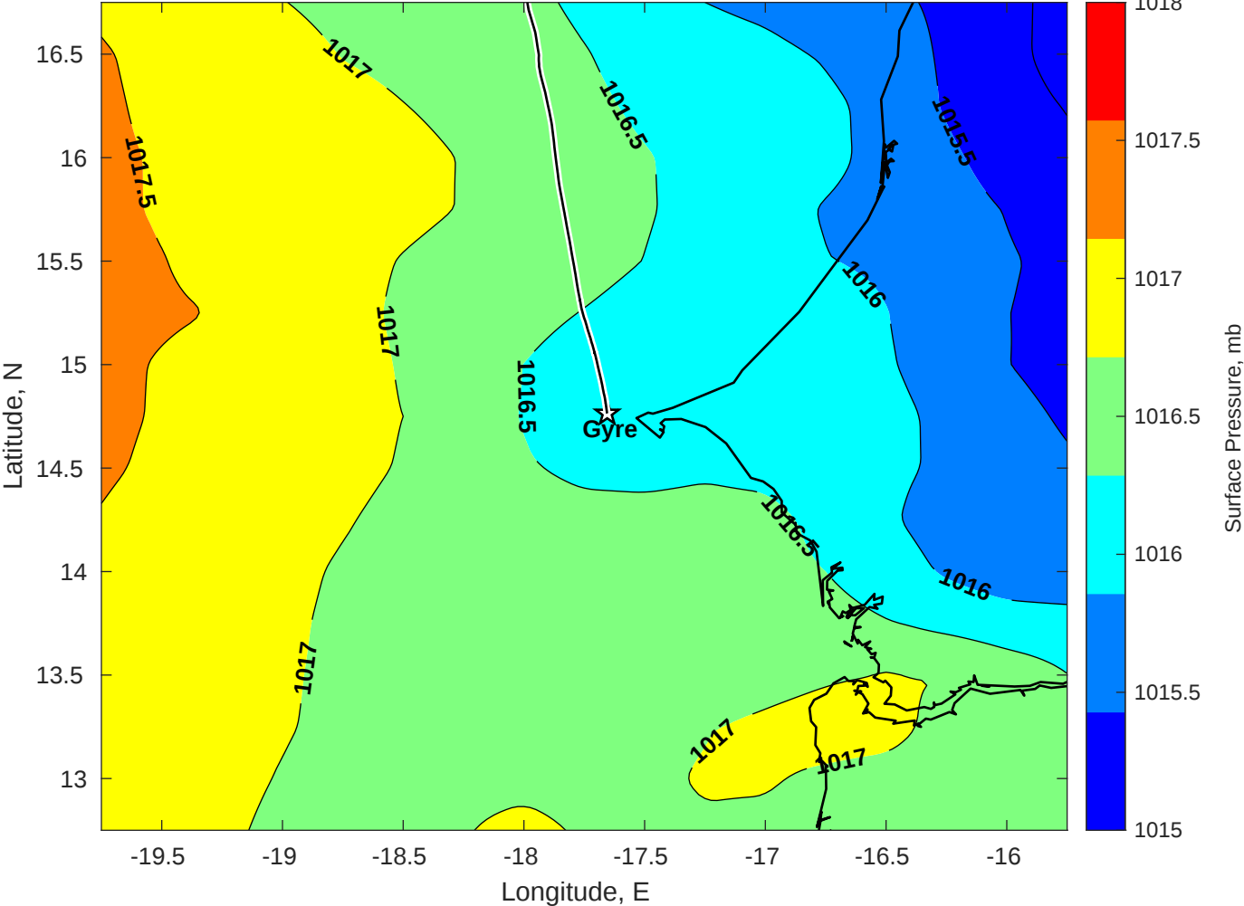
Surface Pressure (mb) for Gyre at 03-Jun-2025 00:00:00
