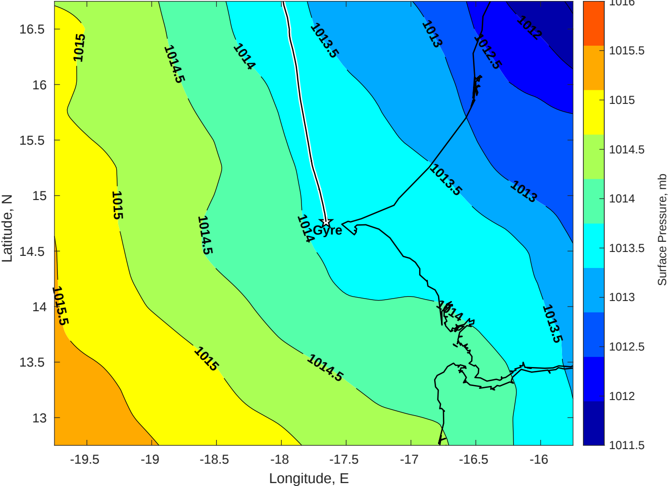
Surface Pressure (mb) for Gyre at 04-Jun-2025 00:00:00
