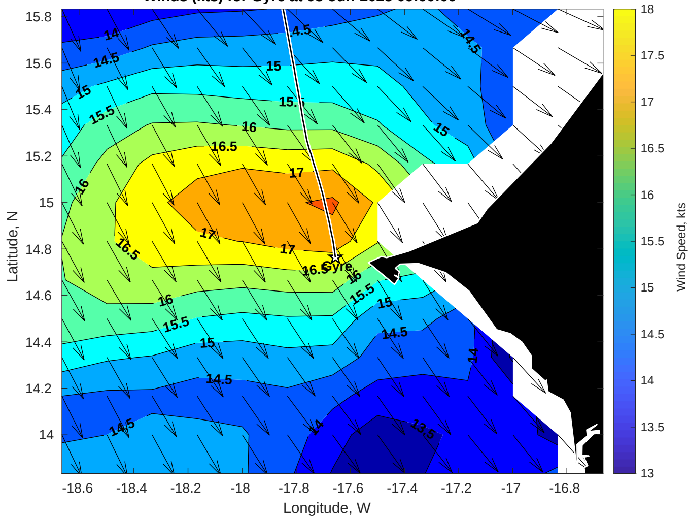
Winds (kts) for Gyre at 03-Jun-2025 09:00:00
