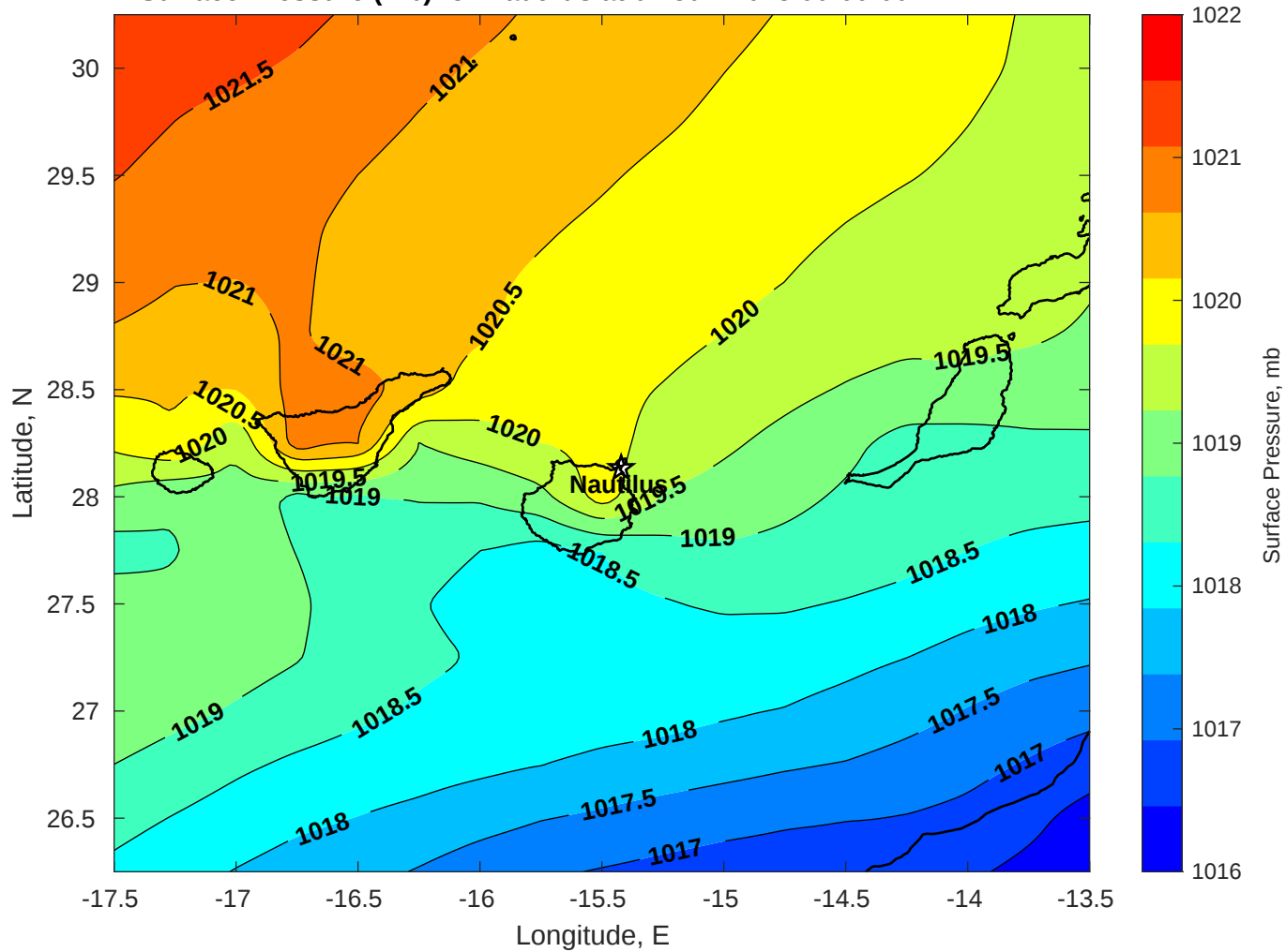
Surface Pressure (mb) for Nautilus at 01-Jun-2025 00:00:00
