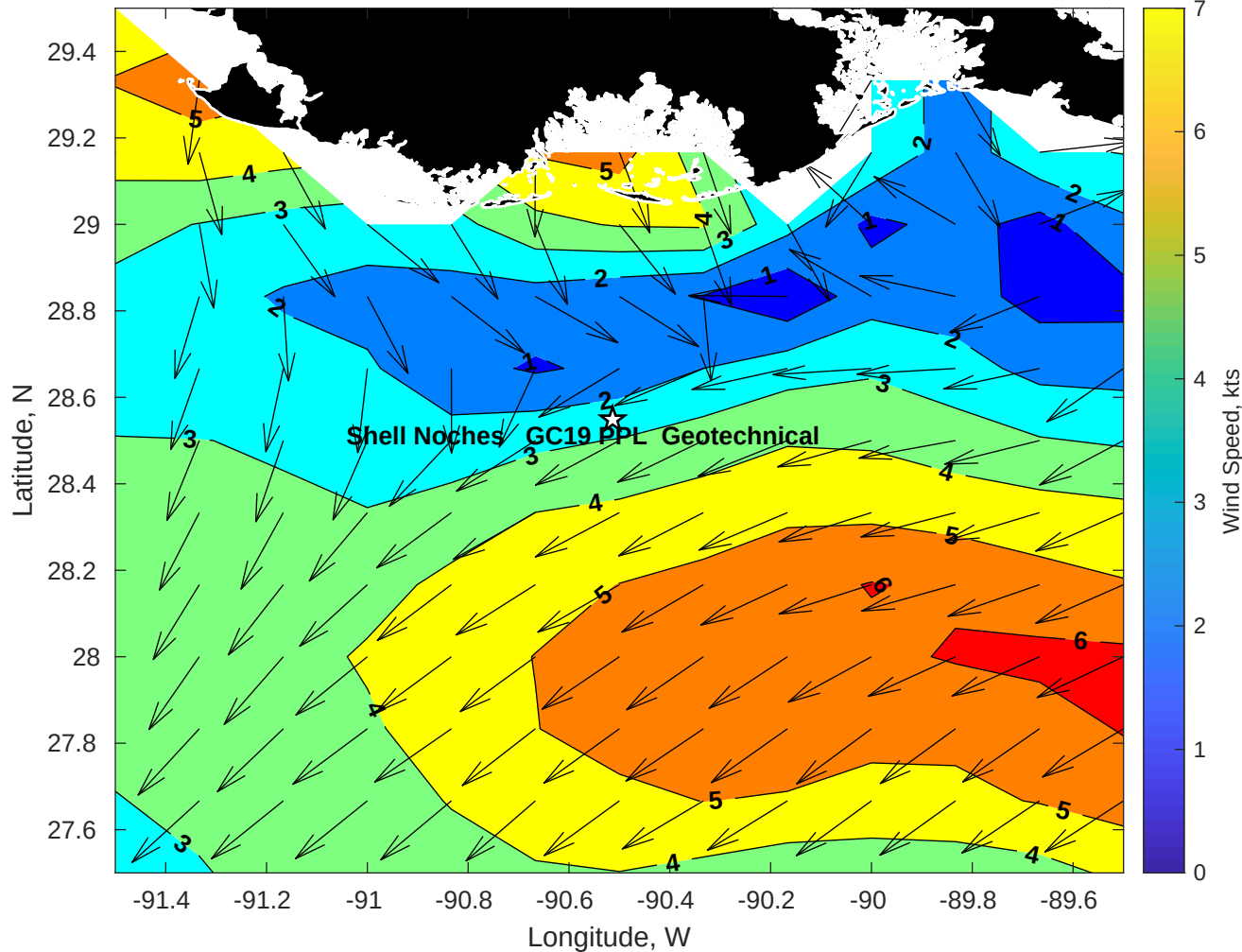
Winds (kts) for Shell Noches GC19 PPL Geotechnical at 01-Jun-2025 09:00:00
