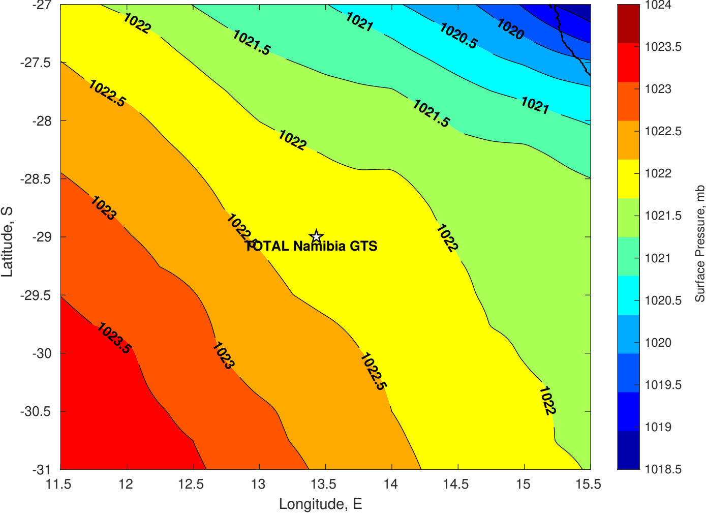
Surface Pressure (mb) for TOTAL Namibia GTS at 02-Jun-2025 00:00:00
