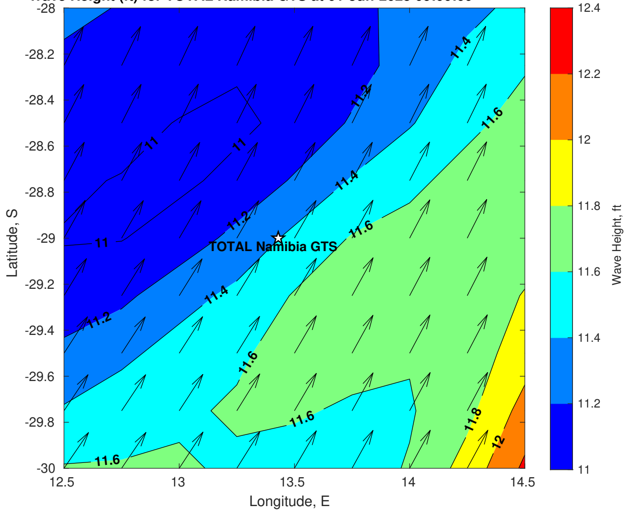
Wave Height (ft) for TOTAL Namibia GTS at 01-Jun-2025 09:00:00
