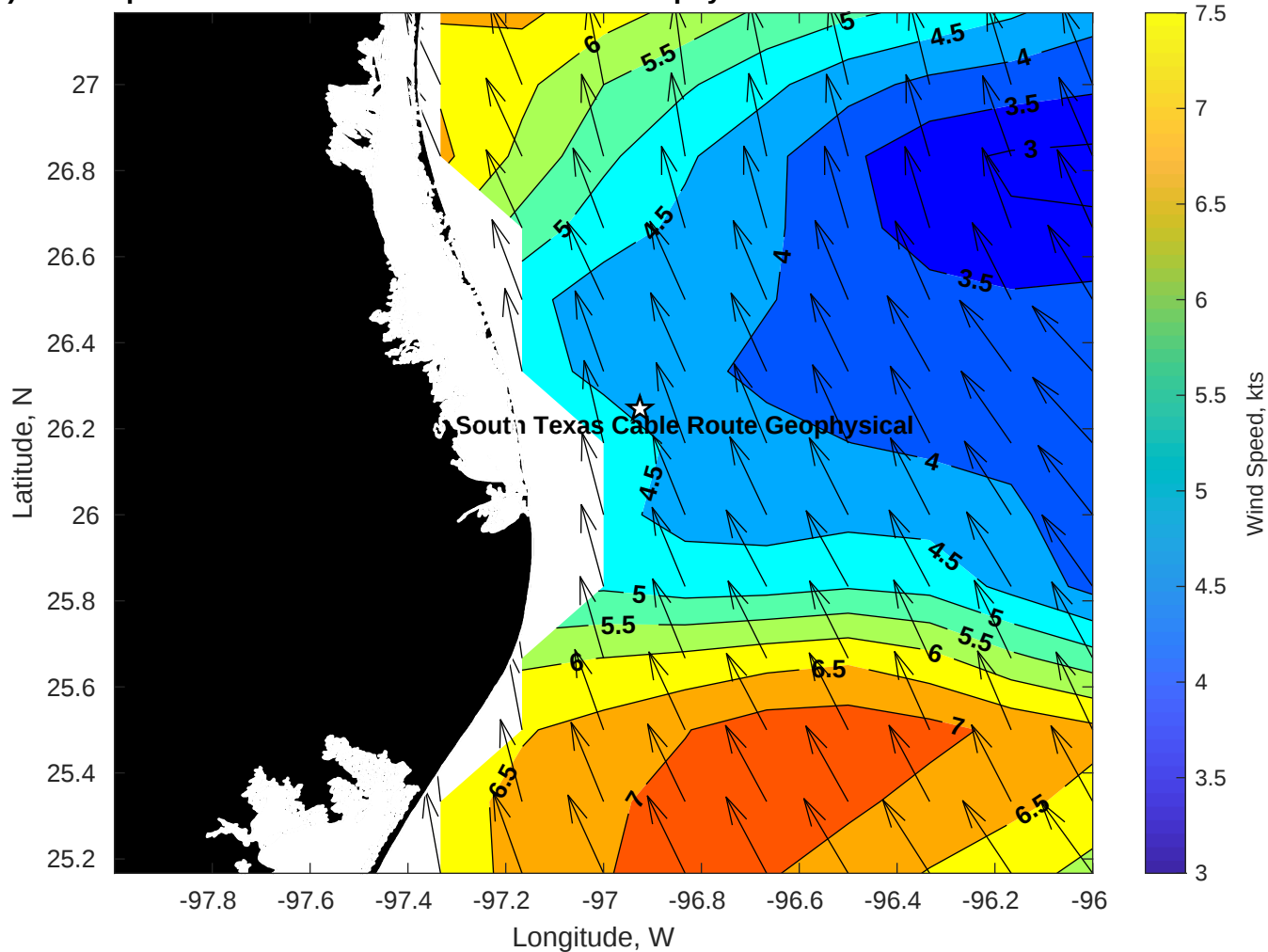
Winds (kts) for Tampnet P2378 South Texas Cable Route Geophysical at 01-Jun-2025 09:00:00
