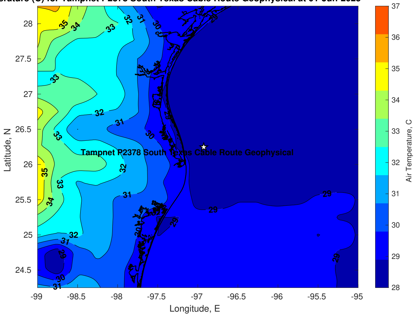
Air Temperature (C) for Tampnet P2378 South Texas Cable Route Geophysical at 01-Jun-2025
