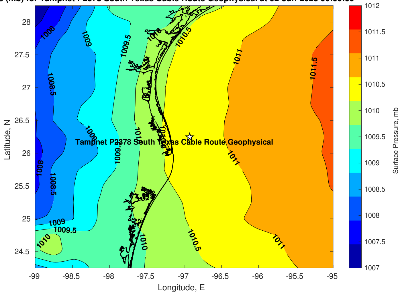
Pressure (mb) for Tampnet P2378 South Texas Cable Route Geophysical at 02-Jun-2025 00:00:00
