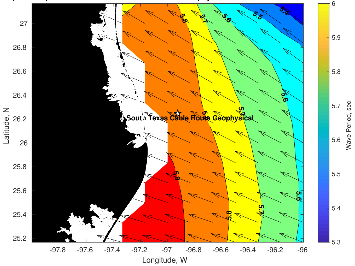
Period (sec) for Tampnet P2378 South Texas Cable Route Geophysical at 01-Jun-2025 09:00:00
