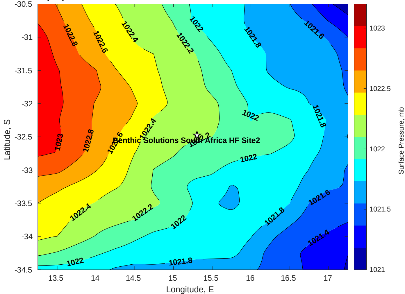
Surface Pressure (mb) for Benthic Solutions South Africa HF Site2 at 02-Jun-2025 00:00:00
