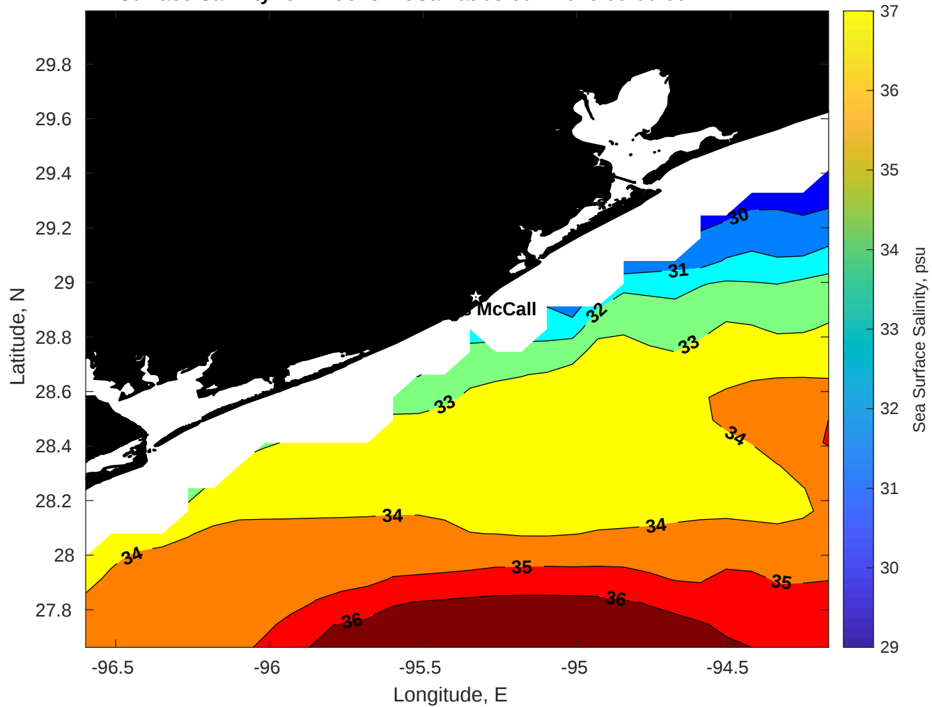
Surface Salinity for Brooks McCall at 03-Jun-2025 00:00:00
