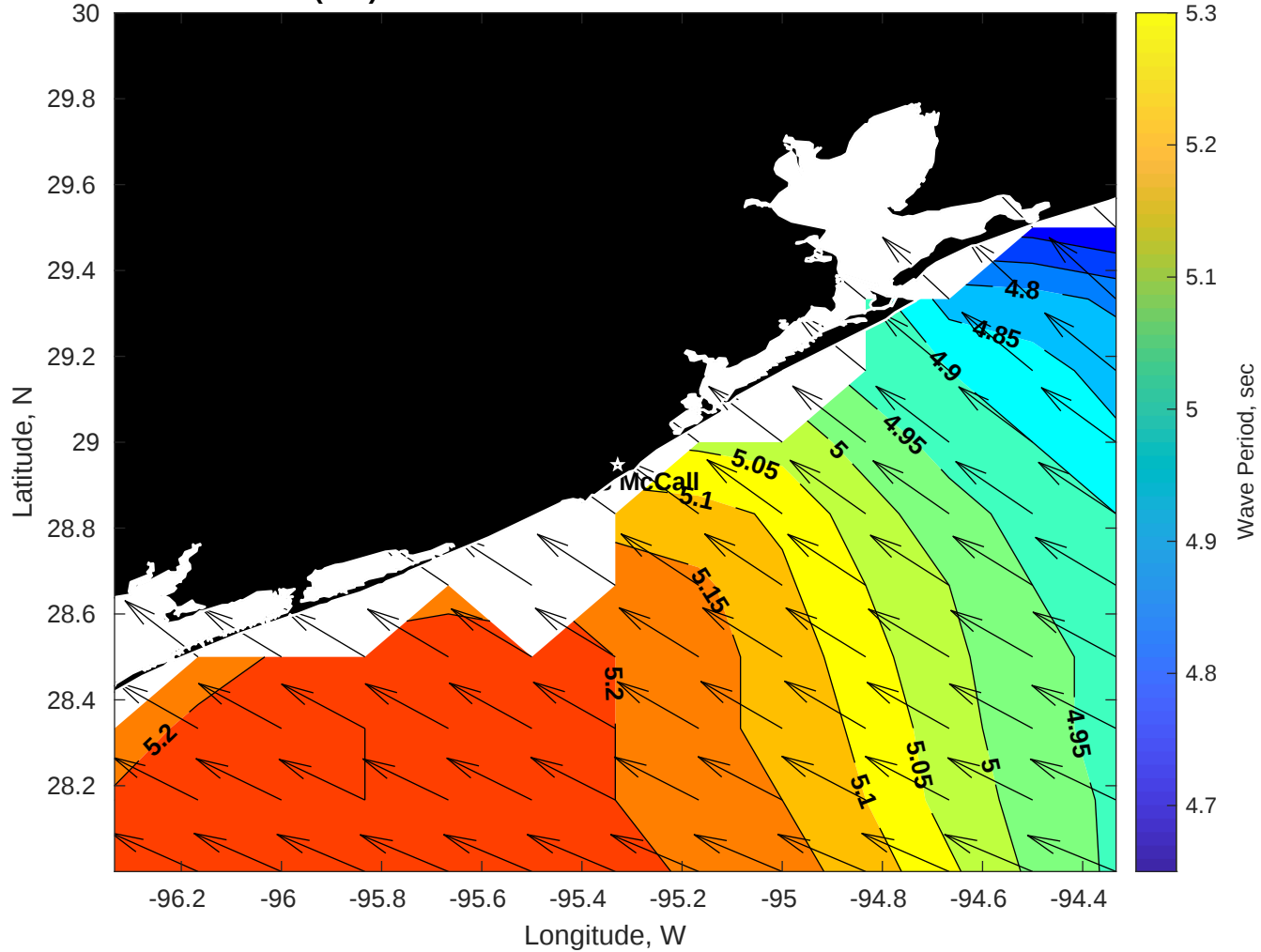
Wave Period (sec) for Brooks McCall at 04-Jun-2025 09:00:00
