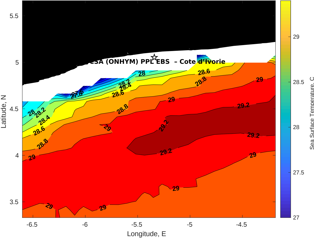
SST for CSA (ONHYM) PPL EBS - Cote d'Ivoire at 26-May-2025 00:00:00
