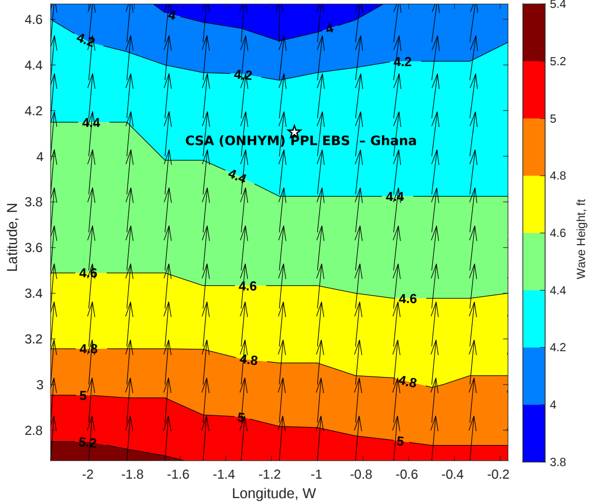
Wave Height (ft) for CSA (ONHYM) PPL EBS - Ghana at 01-Jun-2025 09:00:00
