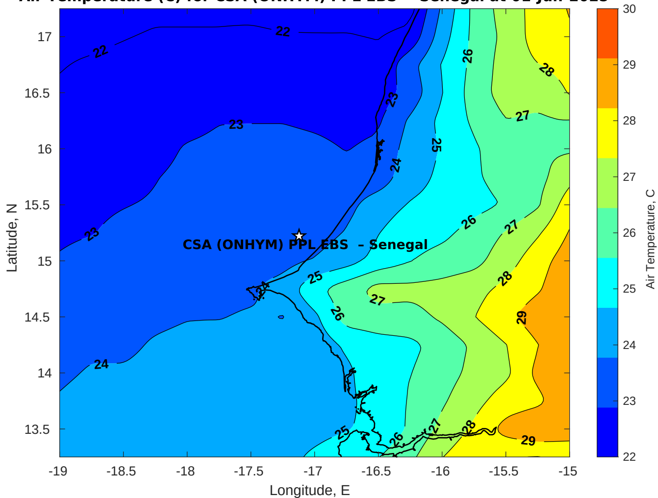
Air Temperature (C) for CSA (ONHYM) PPL EBS - Senegal at 01-Jun-2025
