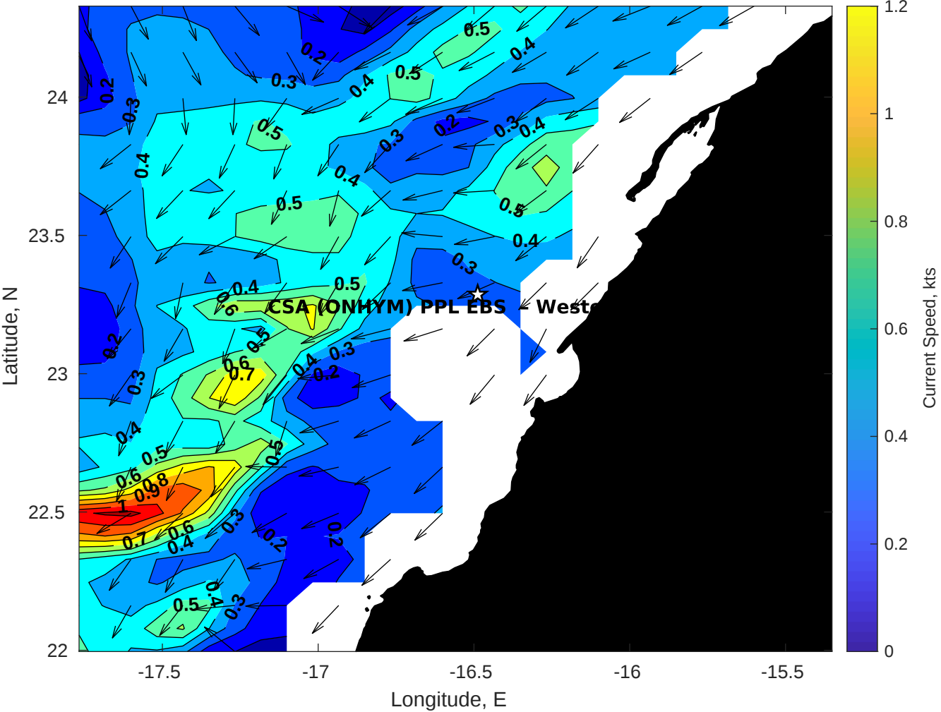
Surface Currents for CSA (ONHYM) PPL EBS - Western Sahara at 26-May-2025 00:00:00
