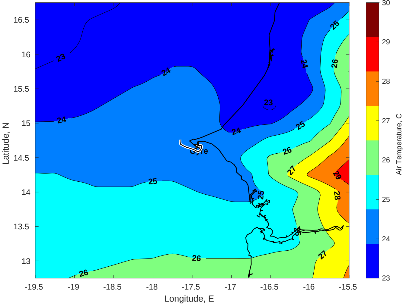
Air Temperature (C) for Gyre at 04-Jun-2025
