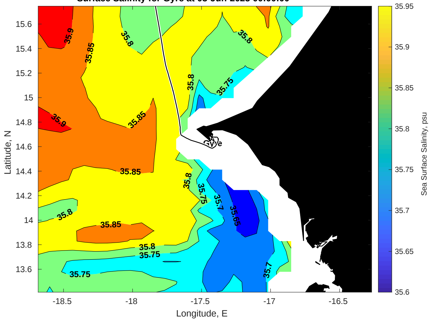
Surface Salinity for Gyre at 03-Jun-2025 00:00:00
