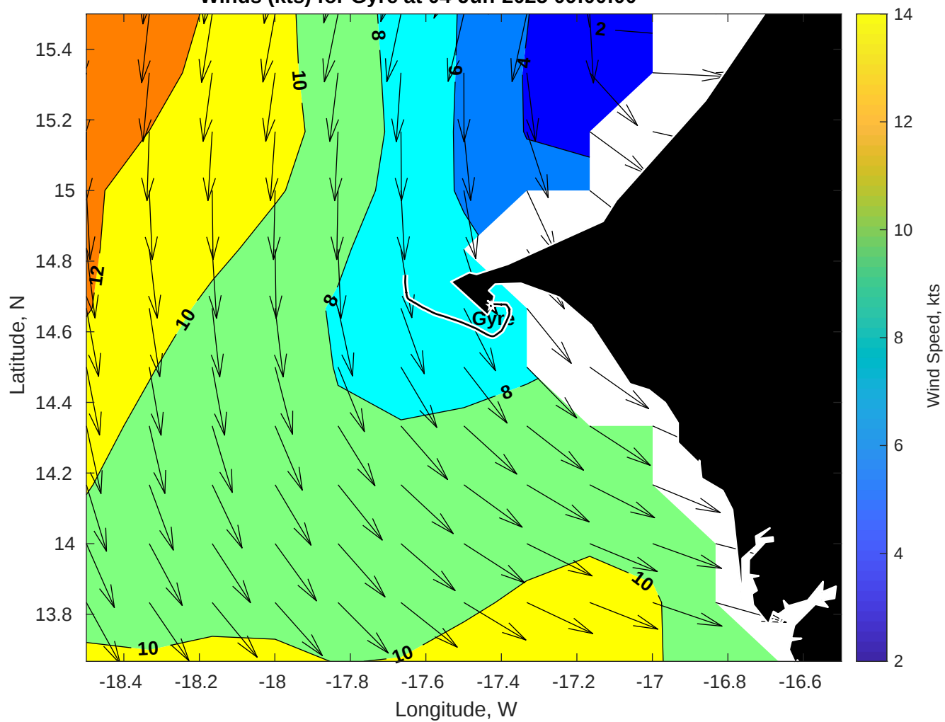
Winds (kts) for Gyre at 04-Jun-2025 09:00:00
