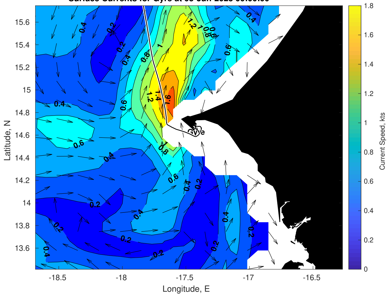
Surface Currents for Gyre at 03-Jun-2025 00:00:00
