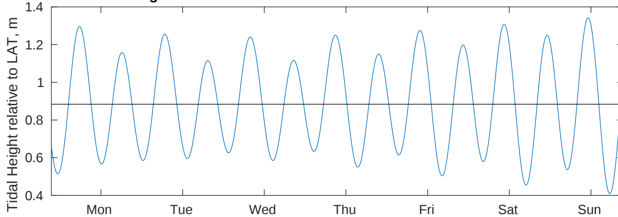
Tidal Currents and Heights for Benthic Solutions South Africa HF Site1 at 20250601
