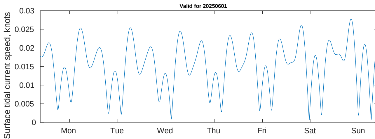
Tidal Currents and Heights for Benthic Solutions South Africa HF Site1 at 20250601
